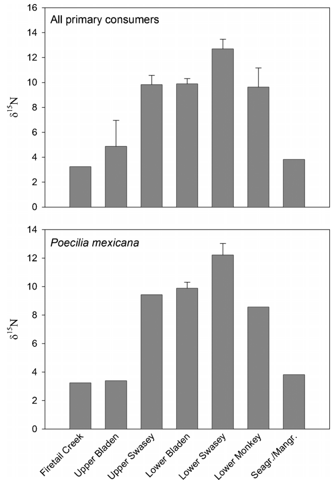
Figure 4. Mean ( \pm 1 S.D.) nitrogen stable isotope signatures of all primary consumer taxa together and Poecilia mexicana alone (the only primary consumer species to occur at all sites). Comparatively higher \delta^{15}\text{N} values of primary consumers at different sites in the same watershed may indicate anthropogenic impacts associated with agricultural land use or human population density
